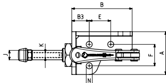
MODEL NO : 511-0-M (KAPLAMASIZ METAL SAP) (UNCOATED METAL HANDLE)
